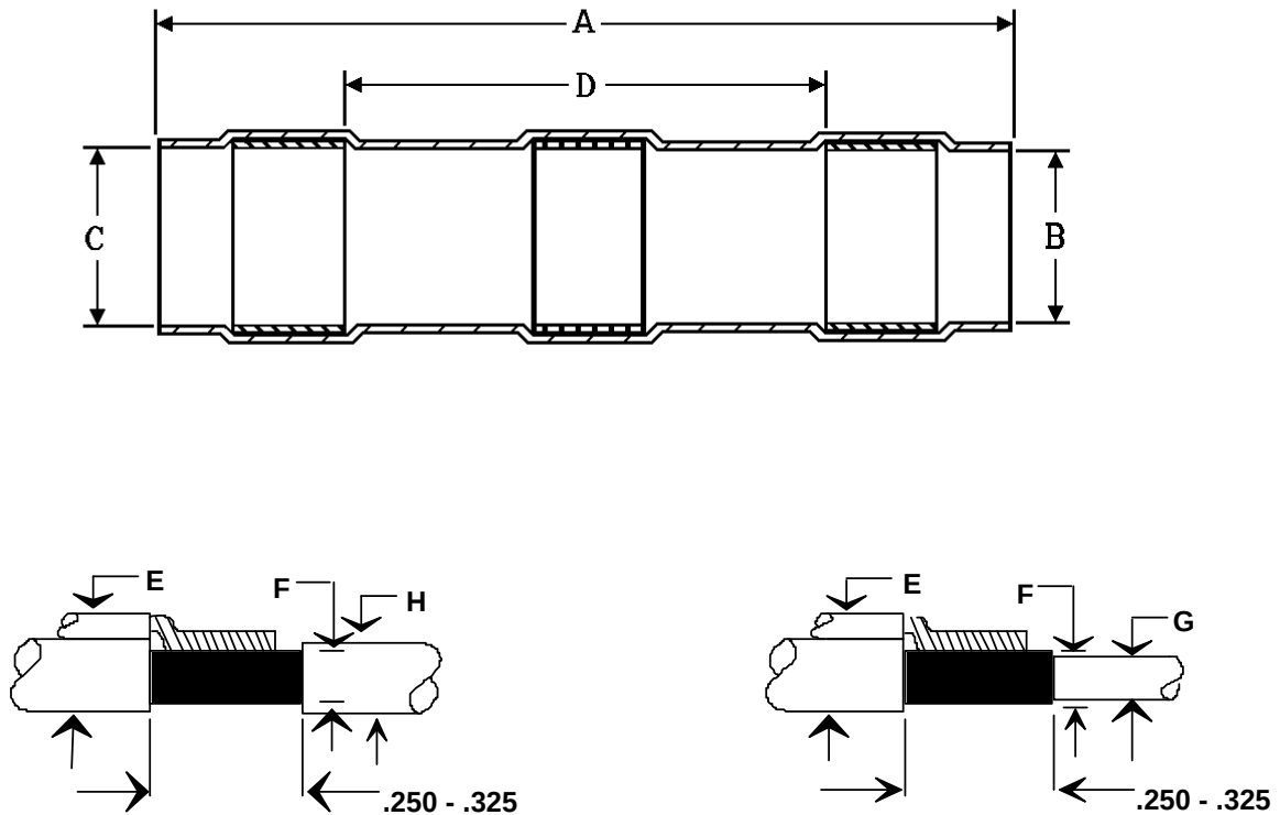
CABLE DIAMETER RANGE AND PREPARATION MEASUREMENTS TABLE 1: Construction details
